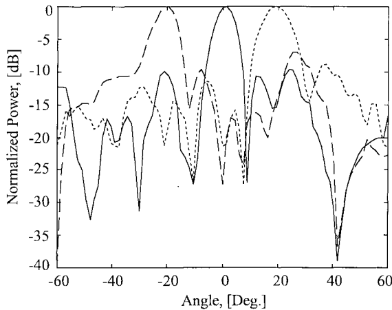
Fig. 13. Beamscanning in E -plane at 10.1 GHz for the 24-element lens amplifier array in receive mode. Receive horn at (—) 0^\circ , (---) -20^\circ , and (···) 20^\circ locations are shown. The normalizing power levels of the main lobes are within 2 dB.
