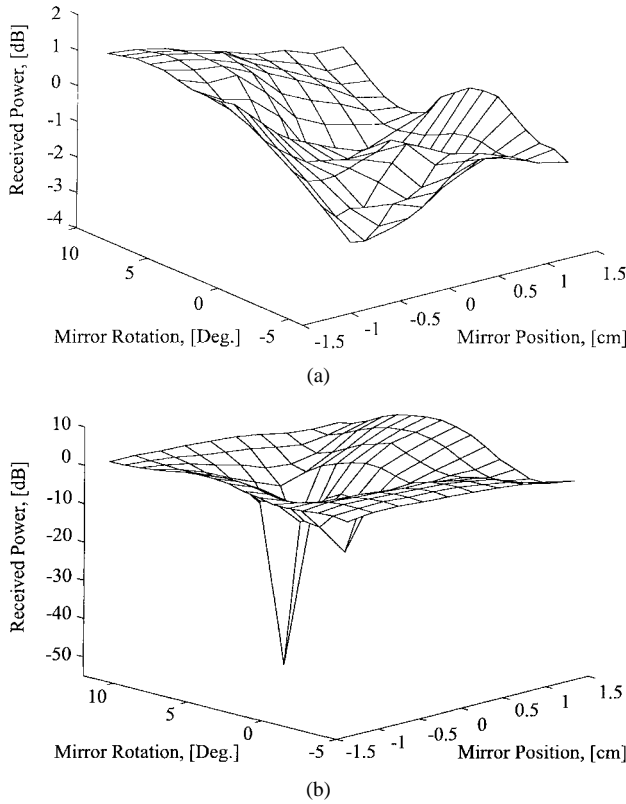
Fig. 12. Measured maximum multipath fading nulls of a 10.1-GHz carrier signal. The received power is normalized to through measurements without the mirror inserted. (a) With and (b) without the 24-element lens amplifier array inserted. Notice the different vertical scales.
