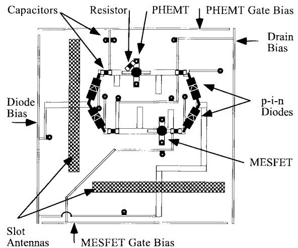
Fig. 2. A bi-directional X-band quasi-optical array amplifier element. The slot antennas are 2.5 cm long and 2 mm wide, and the unit cell dimensions are 3.5 cm \times 3.7 cm.
