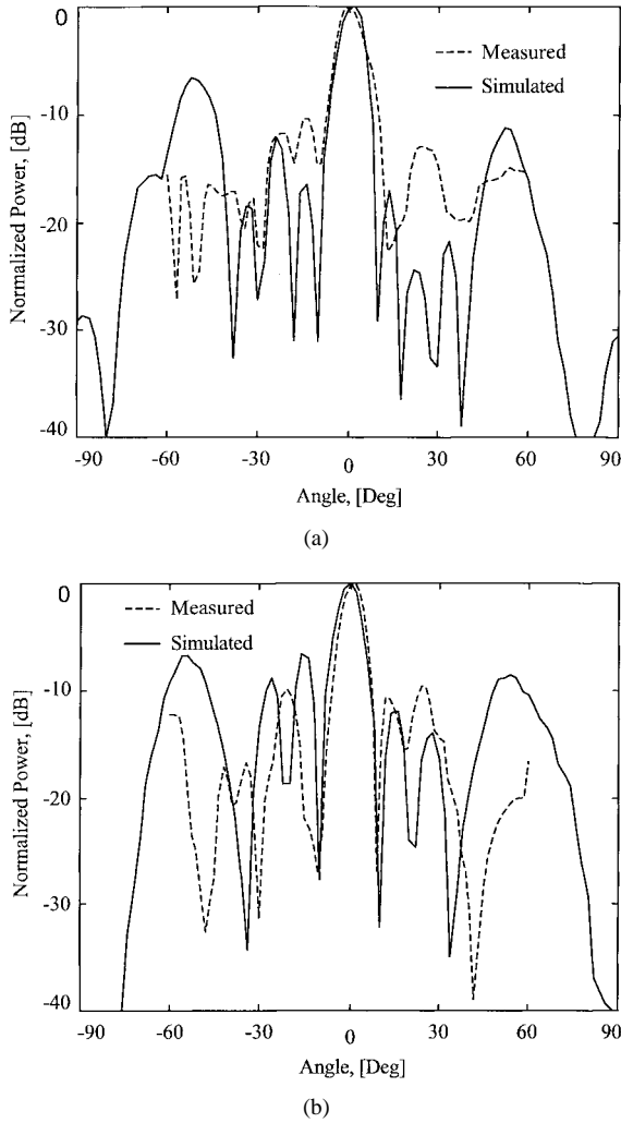
Fig. 9. (a) Measured (---) and simulated (—) H -plane radiation pattern for the receive amplifier at 10.1 GHz. (b) Measured (---) and simulated (—) E -plane radiation pattern for the receive amplifier at 10.1 GHz. The theoretical patterns were calculated using the measured antenna pattern of a single slot antenna.
