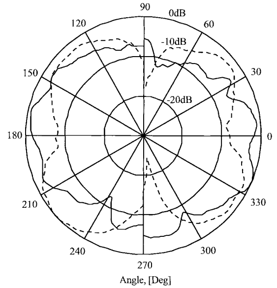
Fig. 5. Measured radiation patterns for a single antiresonant slot antenna at 10 GHz. 0° represents the circuit side and 180° represents the ground plane. E -plane (—) and H -plane (---).
