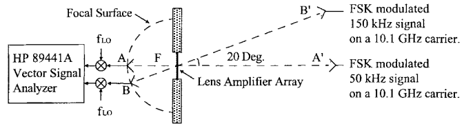
Fig. 14. Test setup for the multiuser experiment. Square-wave signals at f_A = 50 kHz and f_B = 150 kHz are frequency modulated on a 10.1-GHz carrier and input at 0^\circ and 20^\circ from the optical axis, respectively. The two signals are received by horns located on the focal surface behind the 24-element lens amplifier array, and demodulated using a vector signal analyzer.
