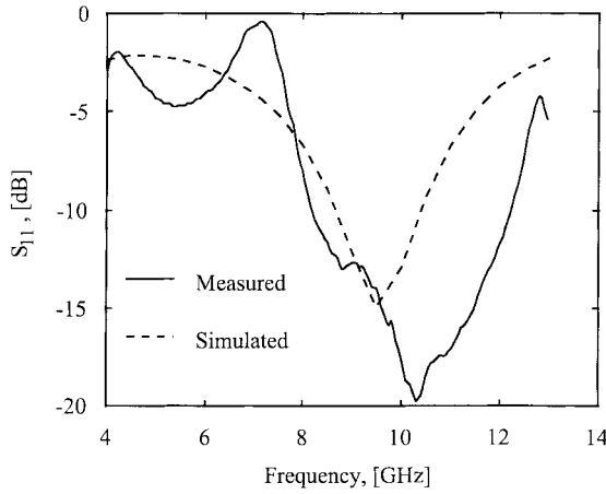
Fig. 4. Measured (—) and simulated (---) return loss for a single slot antenna. The simulations were performed with the computer-aided design (CAD) package Ensemble .
