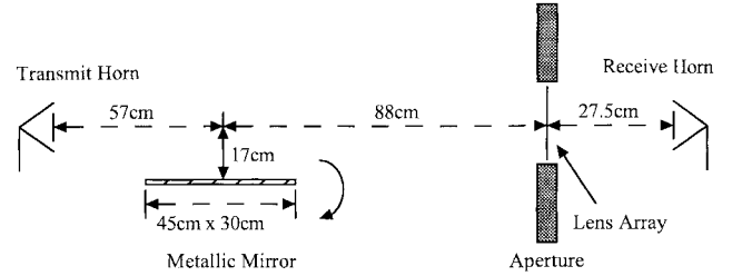
Fig. 11. Test setup for the multipath experiment. A 45\text{ cm} \times 30\text{ cm} metallic mirror located parallel to the optical axis in front of the 24-element lens amplifier is translated in 3-mm steps from the axis. For each step, the mirror was rotated through a set of angles.
