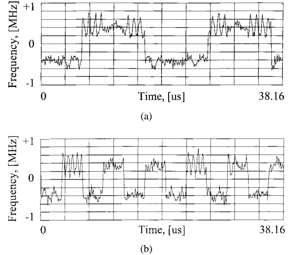
Fig. 15. (a) Received and frequency shift-keying (FSK) demodulated 50-kHz signal for a receiver located at 0^\circ . (b) Received and FSK demodulated 150-kHz signal for a receiver located at 20^\circ . The signals are demodulated using a vector signal analyzer.
