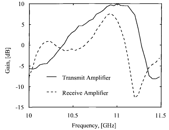
Fig. 6. Measured gain of the transmit (—) and receive (---) amplifier in a unit cell.
