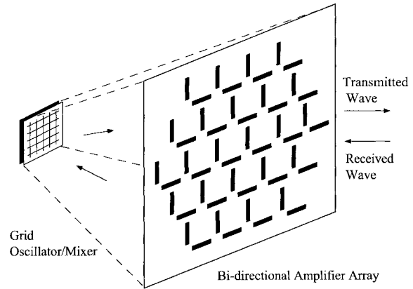
Fig. 1. A quasi-optical T/R module consisting of a bi-directional amplifier and a grid oscillator/mixer.
