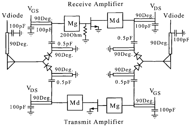
Fig. 3. Circuit schematic of the unit cell. Both amplifiers are matched for gain with matching circuits Mg at the gates and Md at the drains.
