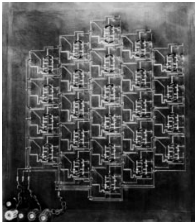
Fig. 7. Photograph of the circuit side of the 24-element bi-directional amplifier array. Orthogonally polarized slot antennas are located in the ground plane, as indicated in Fig. 2.
