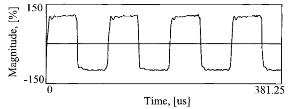
Fig. 10. A 10-kHz square-wave signal received by a quasi-optical receiver front-end and demodulated. A transmitted amplitude modulated 10.1-GHz carrier is received, mixed to a 290-MHz IF, and demodulated using a vector signal analyzer.
