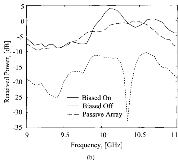
Fig. 8. (a) Measured ON/OFF ratio of the 24-element active and passive array in transmit mode, with polarizers at input and output. (b) Measured ON/OFF ratio of the 24-element active and passive array in receive mode, with polarizers at input and output. The measurements are normalized to a through measurement with a rectangular aperture surrounded by absorbing material. The solid lines represents the biased on state, the dotted lines the biased off state, and the dashed lines shows the measured results for the passive array.
